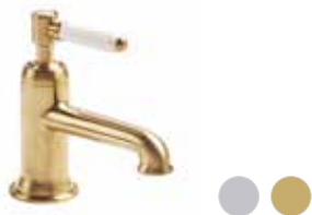
Basin mono basin mixer with click waste 62(w) x 162(h) x 160(d)mm Minimum operating pressure 0.2bar
